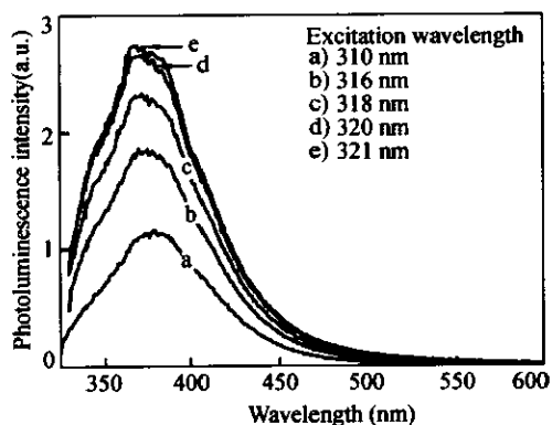
Fig. 2 Intrinsic photoluminescence of PET, \lambda_{ex} = 310 \sim 321 nm
